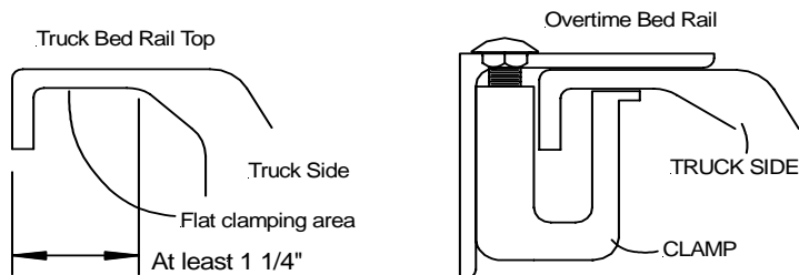
Bed Rail Clamping Clearance
