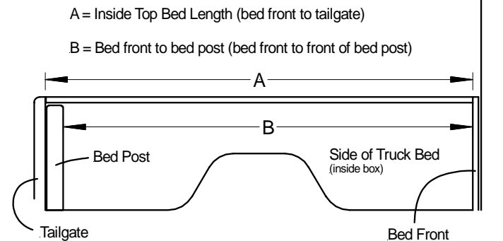
Overtime Bed Rail Fitting Diagram
